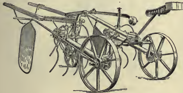
FIG. 3.—Swathe-turner. (Blackstone & Co., Ltd.)
